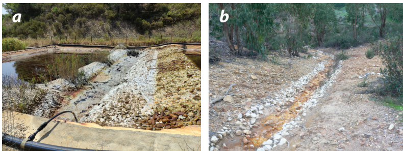
Figure 2. Current state of rehabilitation activities implemented by Empresa de Desenvolvimento Mineiro (EDM) in the RELOUSAL rehabilitation project; a) Degraded artificial wetland system after several decades; b) open limestone channel exhibiting iron oxide encrustation.
