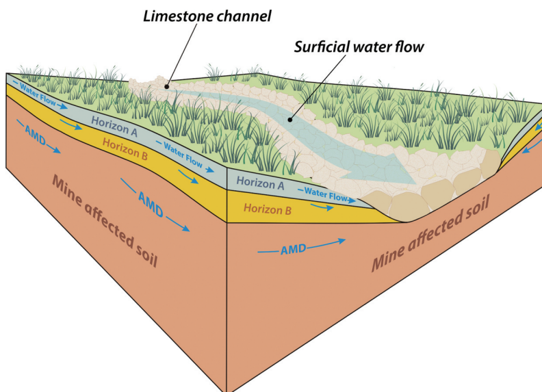
Figure 9. Diagram of the soil cover designed and constructed in the Lousal rehabilitation project.
